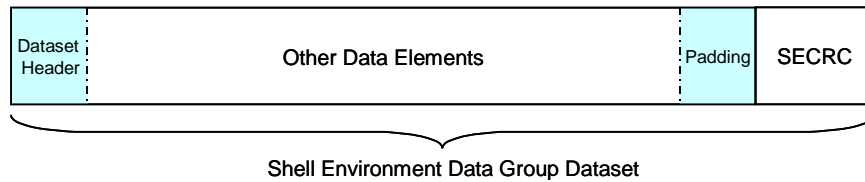
Figure 10 - The ITSO Shell Environment Data Group
