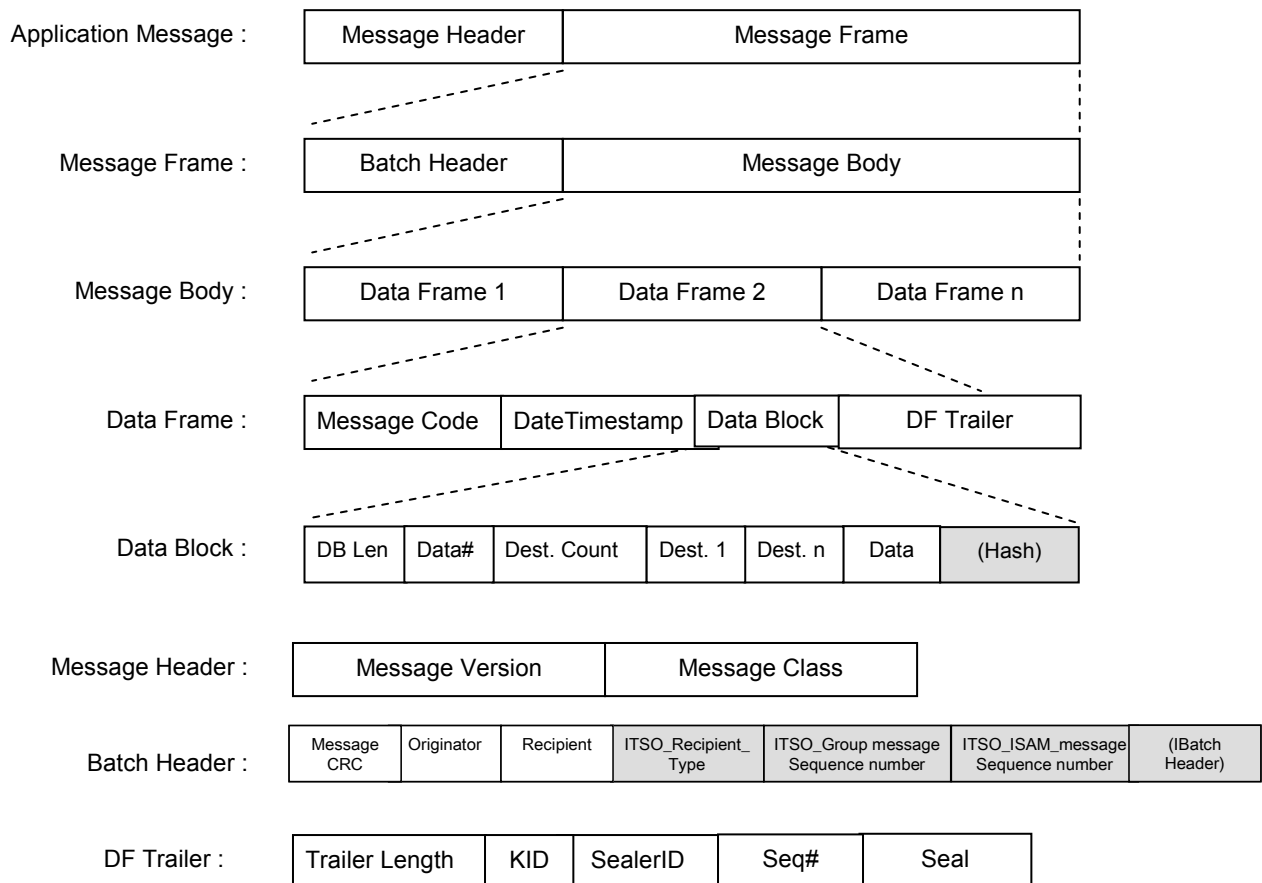
Figure 3 - General application level message structure
